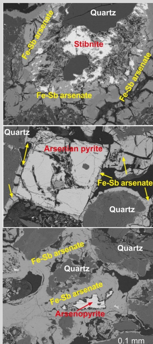
Figure C6. Electron microscope images of cemented arsenate minerals.
