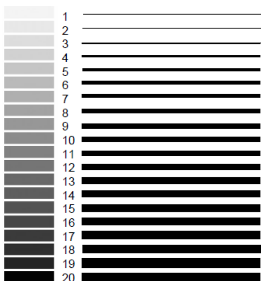
Figure 25. Field turbidity measurement strip for use in conjunction with turbid water in 450 mL clear plastic cups (see Table 5).
