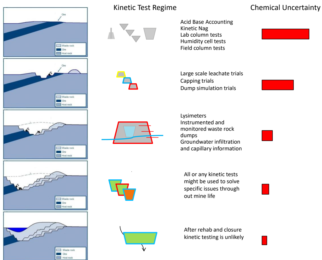
Figure 23. Schematic representation of the hierarchy of kinetic testing.
