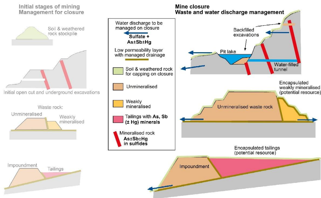
Figure 28. Key features of mesothermal gold mines (on right) that are relevant for rehabilitation and closure, and key potential environmental issues related to water discharge from the various features. Construction of the various features should be done from the opening of the mine (screened, at left), in parallel with closure planning (see Figure 17).
