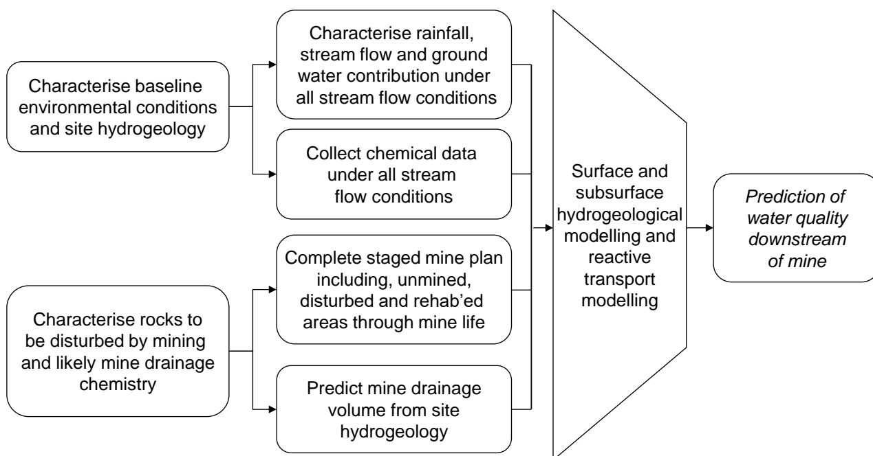
Figure 13. The basic process for determining water quality downstream of a mine.
