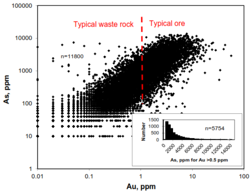
Figure 24. Gold and associated arsenic analyses for Macraes gold mine, Otago, a large, mesothermal deposit. The definition of ore versus waste rock changes with prevailing economic factors. Many waste rock samples analysed have a significant arsenic content (see inset histogram). Management of this material is important for environmental reasons and also because this material may become a resource in the future if the definition of ore changes to lower gold content.
