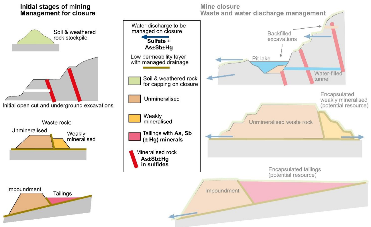
Figure 17. Management of two types of waste rock, and management of tailings, at the outset of mining activity (left) with a view to a closure plan (screened, at right).
