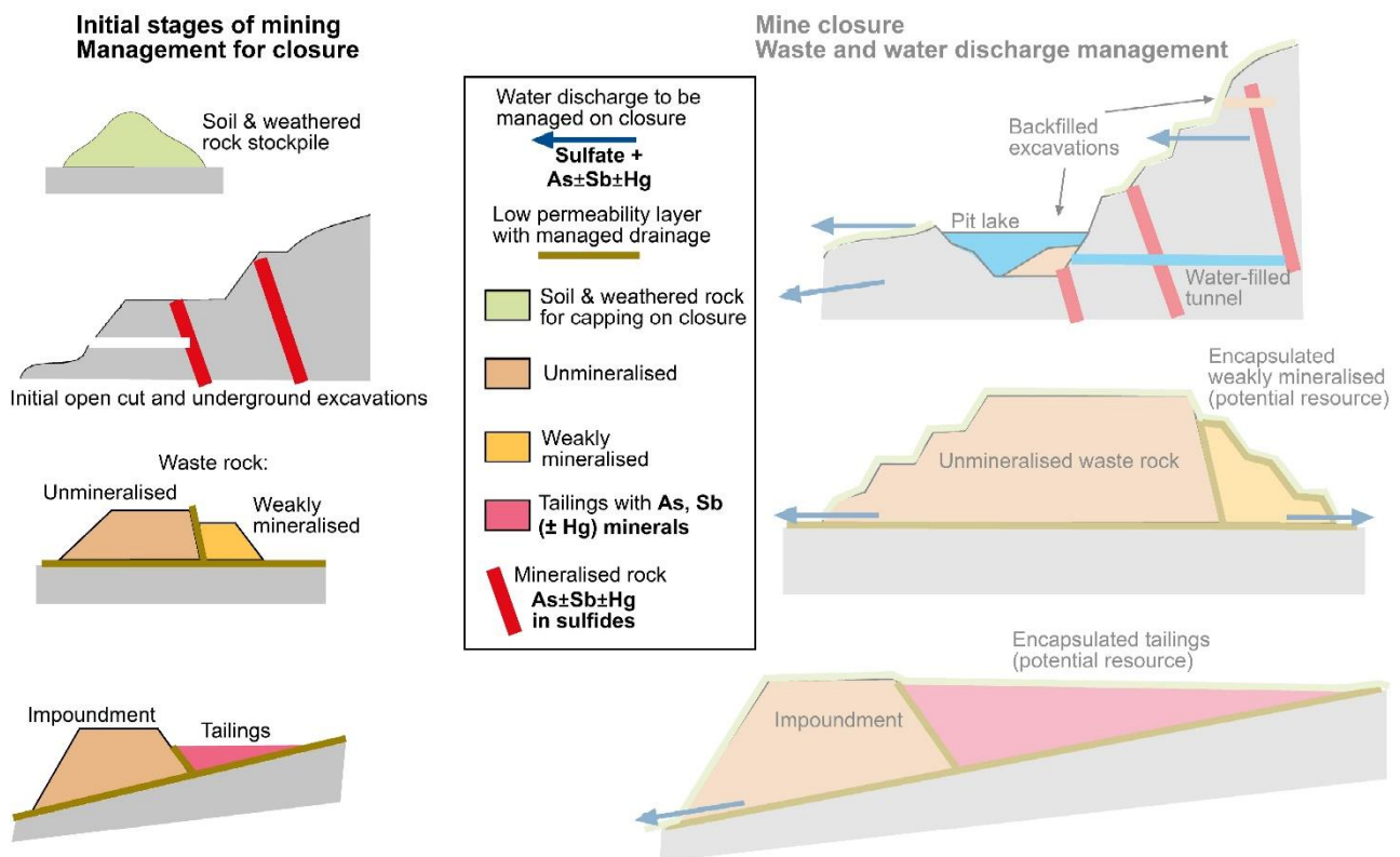
Figure 22. Management of two types of waste rock and management of tailings, at the outset of mining activity (left) with a view to a closure plan (screened, at right).
