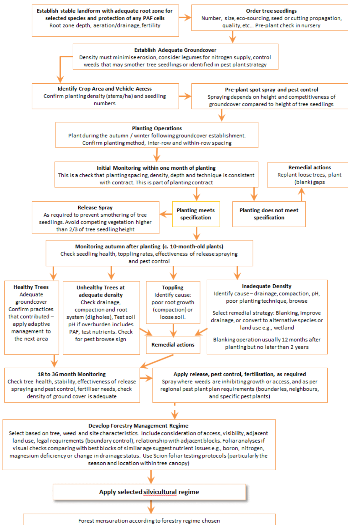
Figure 33. Process for rehabilitating mined areas to production forestry.
