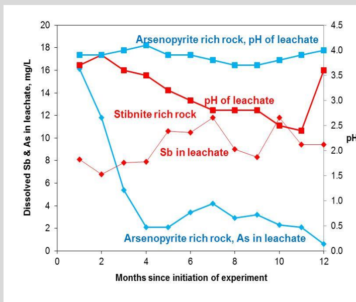
Figure C13. Mobility of As and Sb from leaching of arsenopyrite-rich and stibnite-rich ore material with simulated rainwater.
