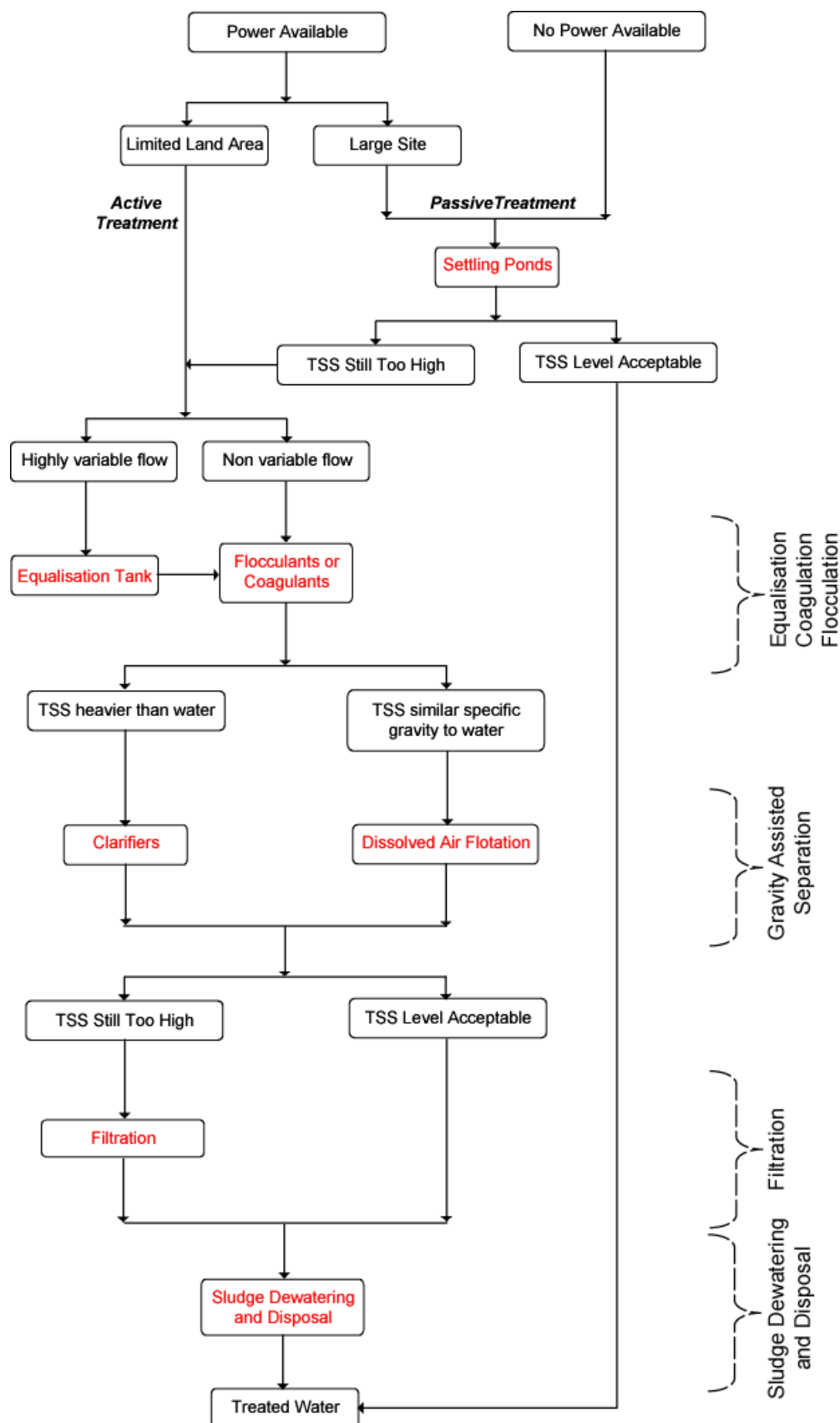
Figure 19. Flow chart to select a treatment system for total suspended solids (TSS).
