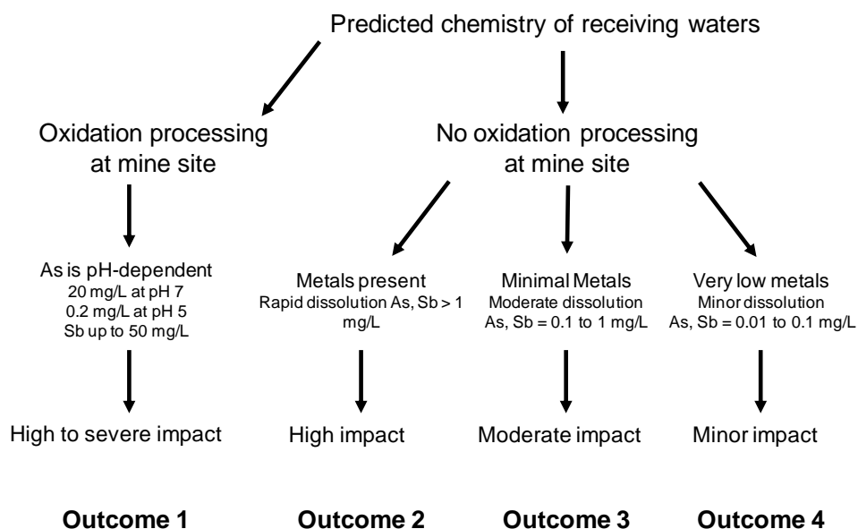
Figure 15. Ecological impact outcomes arising from mesothermal mine drainage based on predicted water chemistries.
