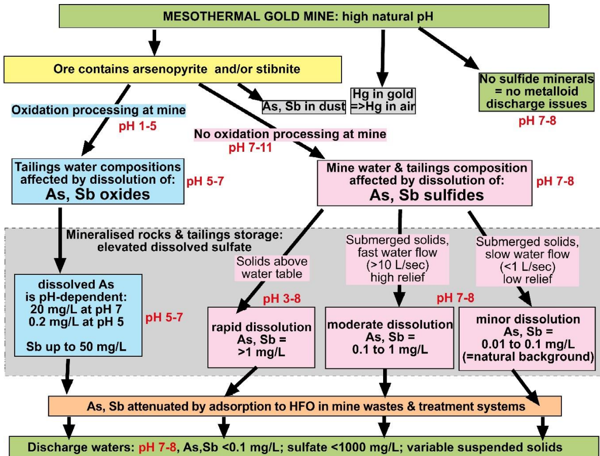
Figure 14. Predicted water quality associated with a mesothermal gold mine, depending on mineralogy of mineralised rock (ore), mine planning and ore processing system, and topography of the site where waste is deposited.
