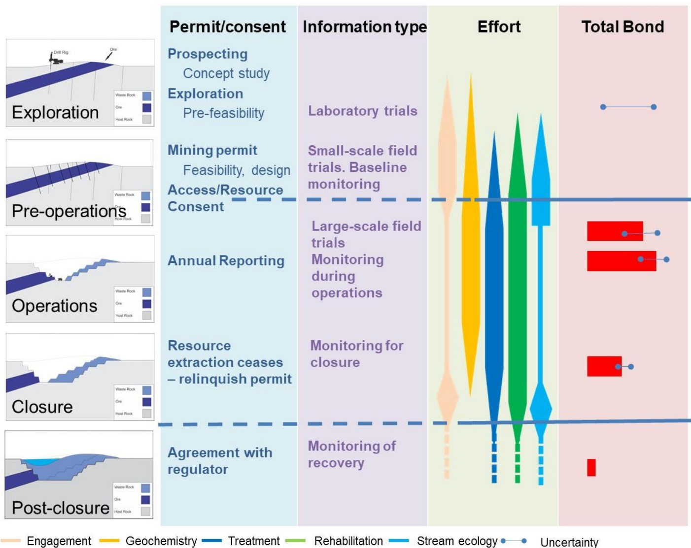
Figure 5. Summary of the relationship between the mine life-cycle, the type of information able to be obtained at each stage of the mine life-cycle (e.g. laboratory studies, field trials), and the focus of effort required in different science streams to reduce the uncertainty associated with the bond.
