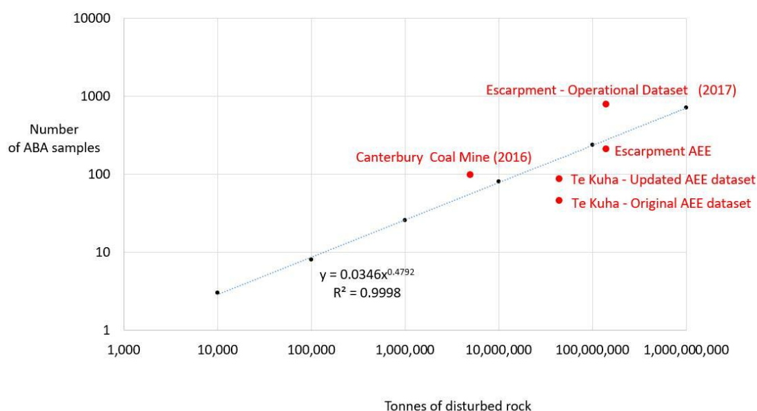
Figure 11. Guideline for number of samples for ABA analysis based on tonnes of waste rock disturbed, and the number of samples collected from different New Zealand mines for assessment of environmental effects (AEE) during operations.
