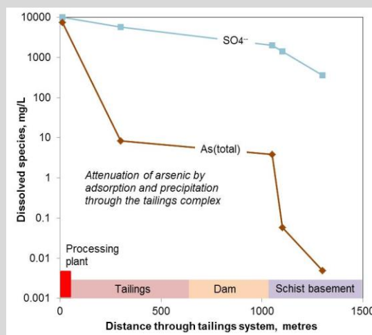
Figure C29. Dissolved As in water as it moves through the tailings complex.
