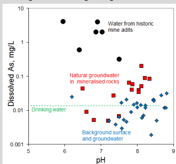
Figure C27. Dissolved As in groundwater at the Macraes mine.
