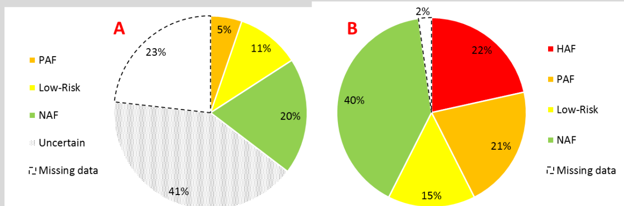
Figure C10. Escarpment coal mine waste rock geochemical classification using the process flow approach. Sulphur values are wt%.
