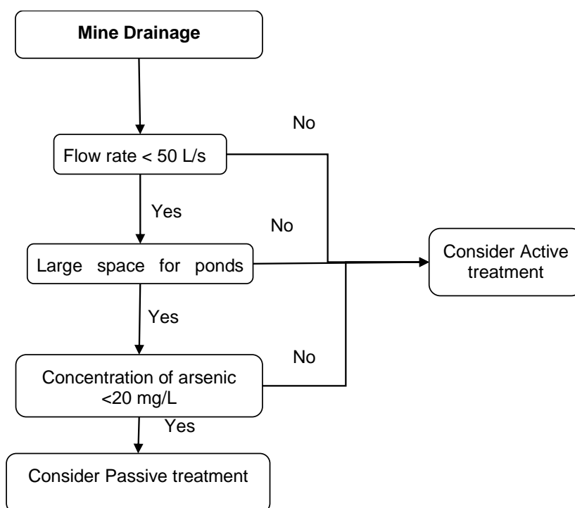
Figure 18. Selection of passive or active treatment for As removal.
