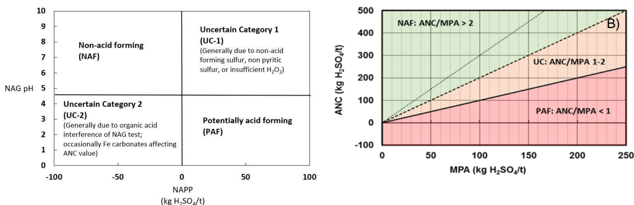
Figure 12. A: NAG pH vs NAPP graph. Samples that are acidic according to both NAG and NAPP tests plot in the PAF field, while those that are non-acidic in both tests plot in the NAF field. Samples where one of the analyses indicates acidic and the other indicates non-acidic plot in the uncertain field and require further investigation. B: ANC vs MPA graph. Material with an ANC:MPA < 2 ratio are classified as non-acid forming material, while ANC:MPA < 1 indicates potentially acid-generating material. If the ANC:MPA is between 1 and 2, the sample classification is uncertain (source: Olds et al. 2015).
