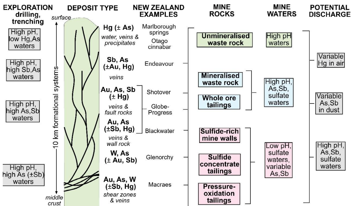
Figure 10. Summary of the principal environmental issues associated with mesothermal gold deposits. The metal/metalloid contents of the deposits are a result of differing levels of original emplacement in the Earth's crust. Subsequent erosion has exposed deposits from different crustal levels at the present surface. These original geological differences affect potential environmental issues at all stages of exploration and mining. Typical New Zealand examples of each deposit type are indicated, and more information on these is included in the references list below.
